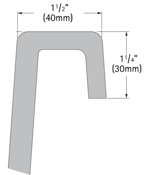
Typical Rim Section
